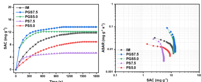
Figure 4 (a) SAC value as a function of desalination time and (b) Kim-Yoon plot for CDI process using different MCDI electrodes (Applied voltage: 1.2 \text{ V} , flow rate: 10 \text{ mL}\cdot\text{min}^{-1} )
