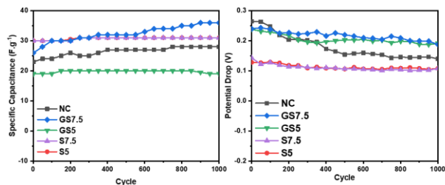
Figure 3 (a) Specific capacitance and (b) potential drop of different MCDI electrodes after 1000 cycles at current density of 0.5 \text{ A g}^{-1} calculated from GCD plot
