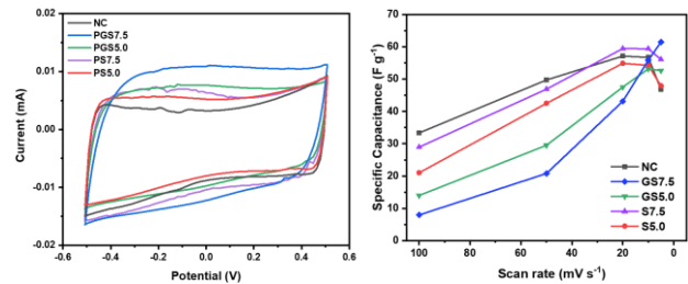
Figure 2 (a) CV plots at scan rate of 5 mV·s -1 and (b) specific capacitance value at different scan rate of different MCDI electrodes
