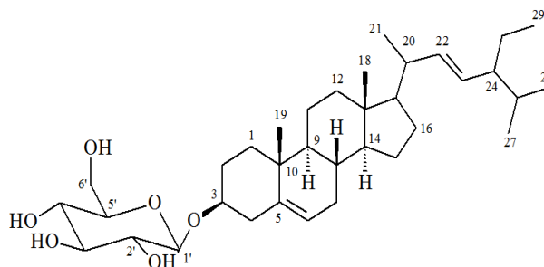
Hình 2 Stigmast-5,22-dien-3-O-β-D-glucopyranoside (2)
