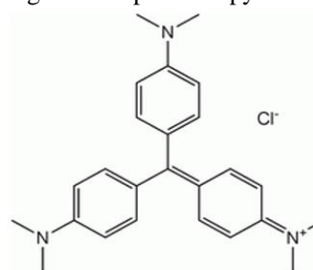
Fig. 3 The chemical formula of crystal violet
